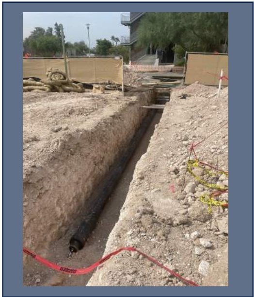
Chilled water piping trenching and installation
